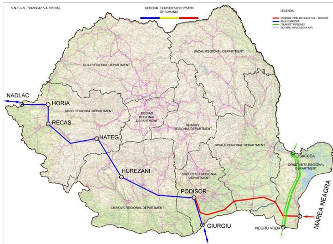
Black Sea Shore – Podisor pipeline route
